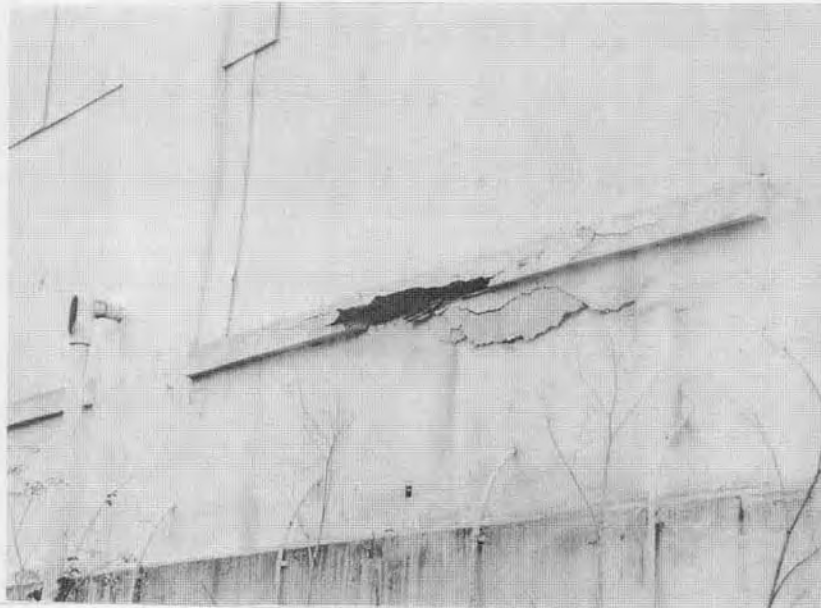
7-5 Powerhouse neglect, deterioration
