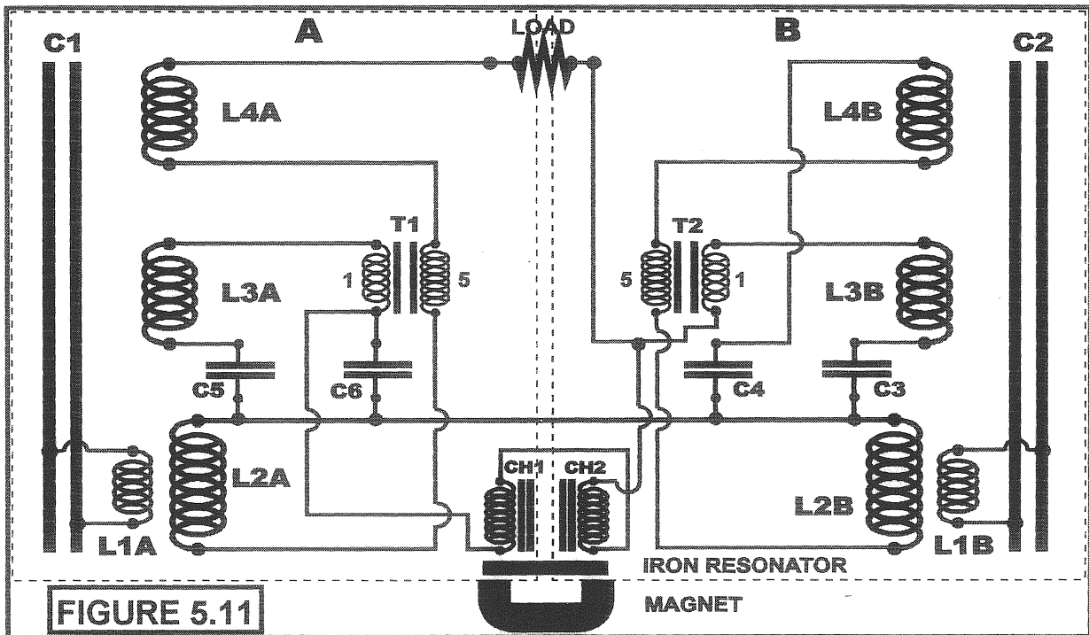
Redrawn Aho Circuit from Figure 5.7
