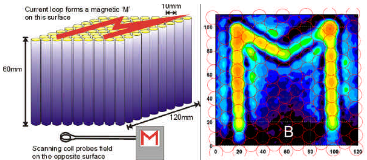
Figure 5. Left: a stack of 10mm diameter Swiss rolls on resonance at 21MHz behaves like a set of 'magnetic wires' conducting magnetic field lines just as a normal electric wire conducts electric field lines. Current loops in the form of an 'M' were placed at one end of the sample and the transmitted field measured by a probe coil. Right: the experimental results of a scan by a probe coil (dimensions marked as in mm). The wavelength at 21MHz is 15m and therefore we are in the extreme near field limit, imaging details on a scale less than 1/1000^{\text{th}} the wavelength.
