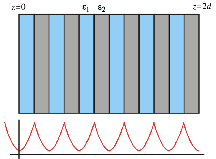
Figure 2. Top: a simple metamaterial comprising alternate layers of a metal such as silver and a dielectric. The layers are presumed to be very thin, much less than the wavelength of light. Bottom: the schematic electric field intensity in the metamaterial showing how a chain of surface plasmon excitations conveys the field from one end of the material to the other.
