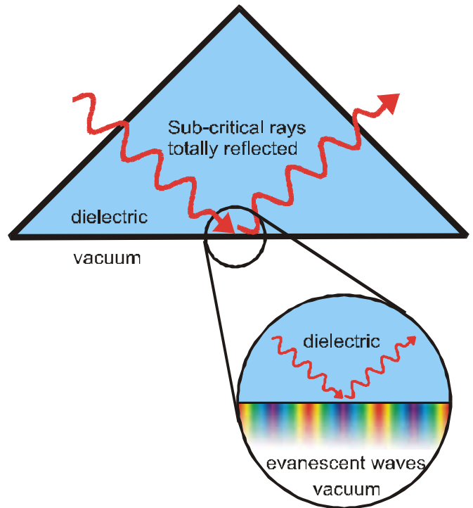
Figure 1. When light is totally internally reflected from a dielectric/vacuum interface, the field in the vacuum is not zero, but dies off rapidly away from the interface. This is an example of the near field.
