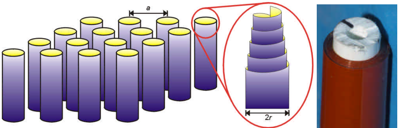
Figure 4. A magnetic metamaterial comprising a sheet of conductor such as copper coated with an insulator and wound around a cylinder. The inductance of the coil and the capacitance between the inner and outer turns produce a resonant circuit. Tuning the frequency through the resonance changes the phase of the response so that a structure consisting of many rolls stacked together is a magnetic metamaterial. On the right we see a realisation of the 'Swiss roll' with a diameter of 10mm and a resonant frequency of 21MHz.
