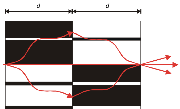
Figure 3. Two media annihilate one another in an optical sense if \epsilon, \mathbf{m} in one is the negative mirror image of \epsilon, \mathbf{m} in the other. Here we show the trajectory of an electromagnetic ray with the second medium correcting for the diversion created by the first.
