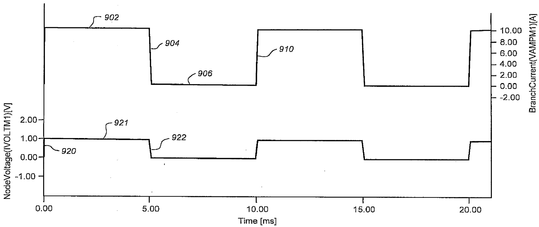
Fig - 9A Windings - Reluctance Switches 1&4
