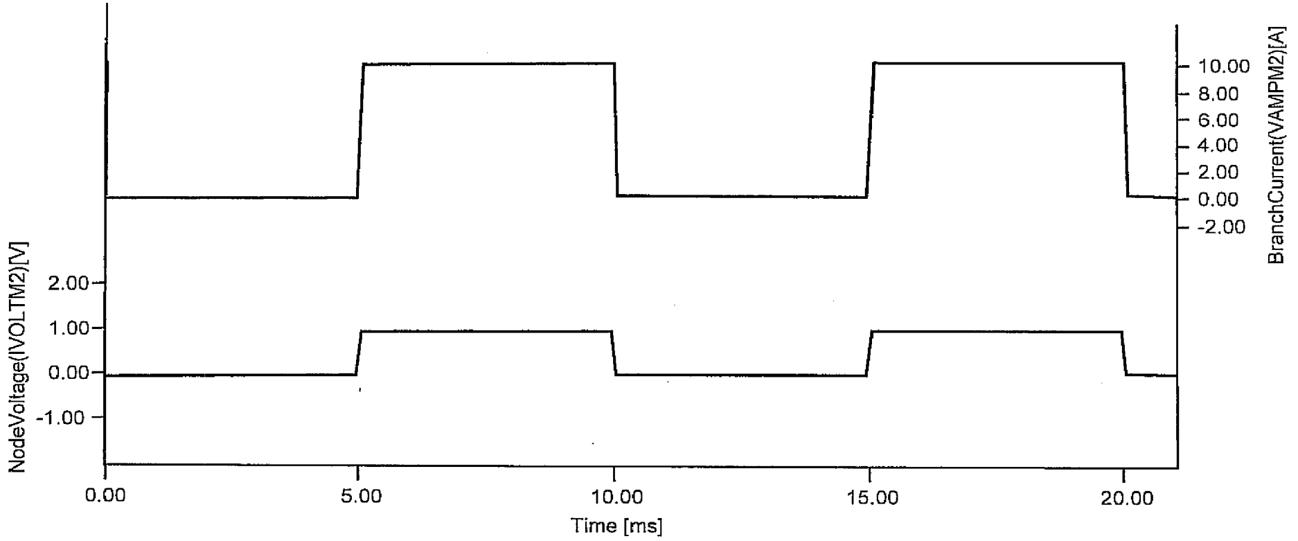
Fig - 9B Windings - Reluctance Switches 2&3
